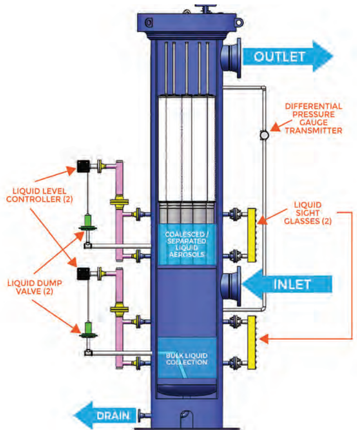
Figure 11 FTC Cyphon Series High-efficiency Gas Coalescer Vessel
