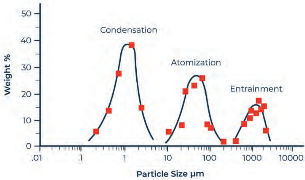
Figure 4 Aerosol Droplet Size by Formation Mechanism 11
