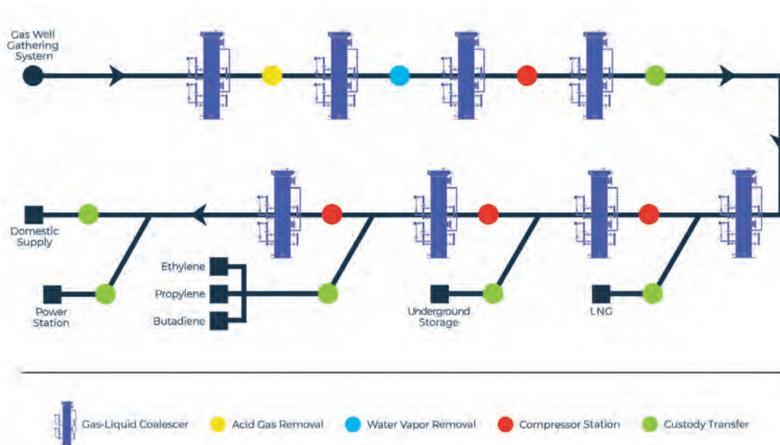
Figure 1 Overview of Gas-Liquid Separation Along the Gas Journey
